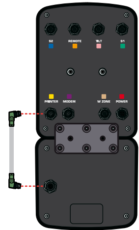
Fig.3 Device and vprint cable connection
