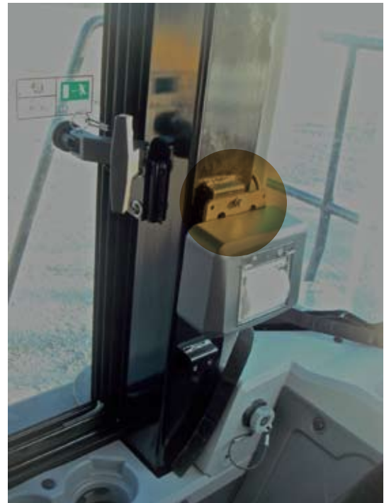
Fig.23 vprint fixed separately on the rear right pillar of a CAT cabin. Pilar provides an holding bracket with holes
