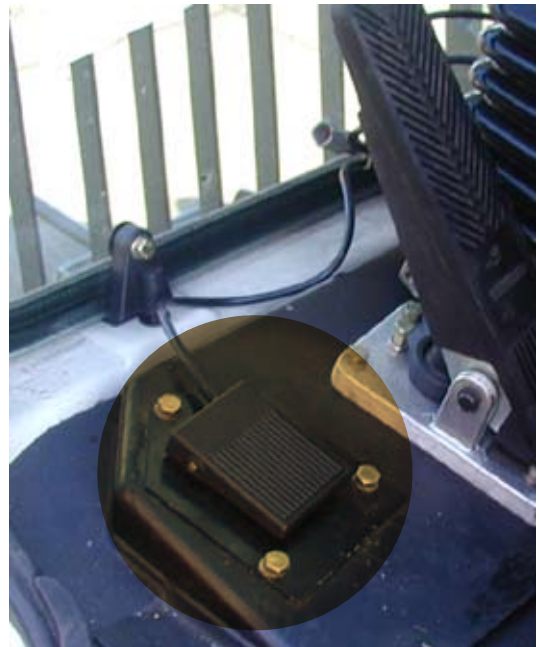
Fig.1 Weighing Pedal
