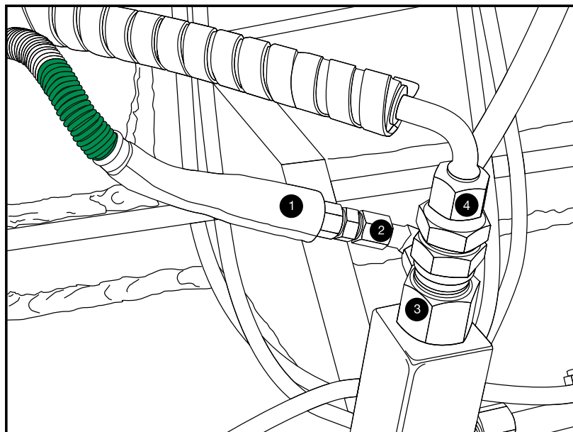
Illustration example of sensor fitting with JIC adapter
